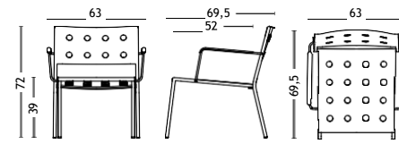
BALCONY LOUNGE ARMCHAIR Width 63 cm Depth 69,5 cm Height 72 cm Seat height 39 cm Seat depth 52 cm
