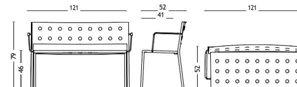
BALCONY DINING BENCH W. ARM Width 121 cm Depth 52 cm Height 79 cm Seat height 46 cm
