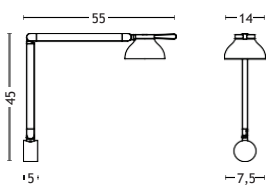
DOUBLE ARM WITH WALL BRACKET WIDTH 14 CM | 5.5" DEPTH 55 CM | 21.7" HEIGHT 45 CM | 17.7"
